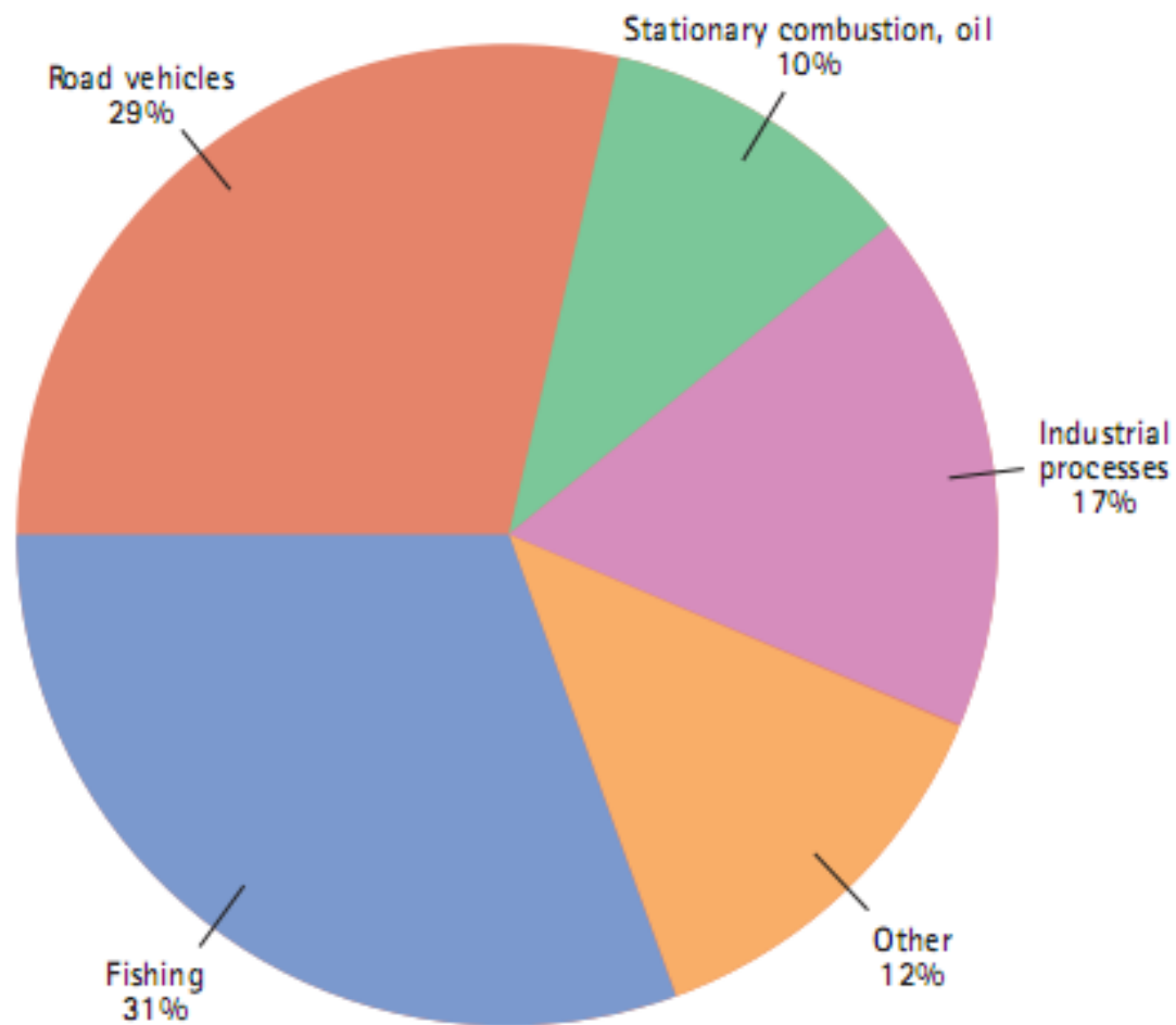
Figure 2.3.2c. Distribution of CO 2 emissions by source in 2003
